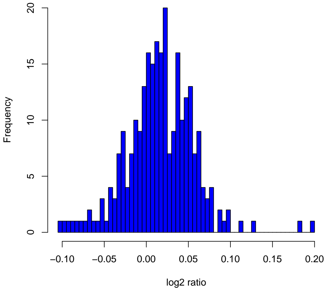
Histogram of log2ratios in 270 HapMap samples at clone Chr15tp-3B10
