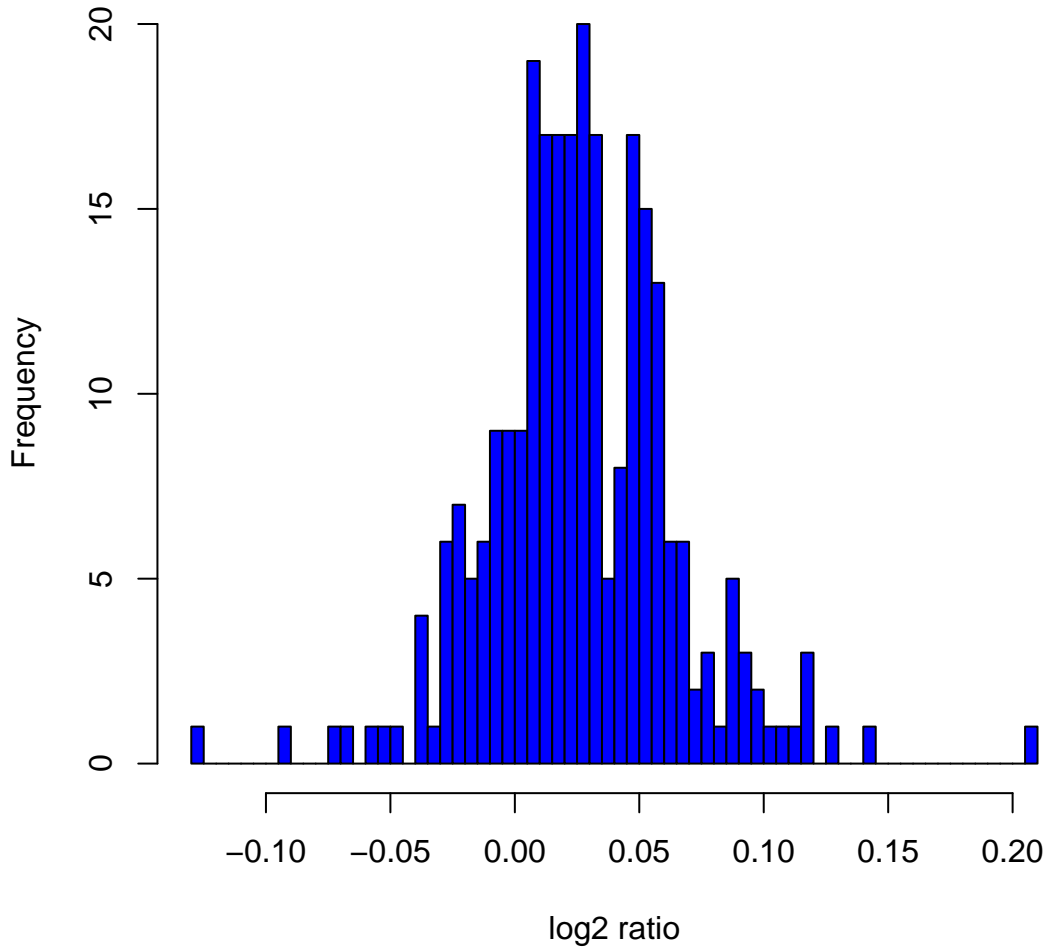
Histogram of log2ratios in 270 HapMap samples at clone Chr15tp-3E11
