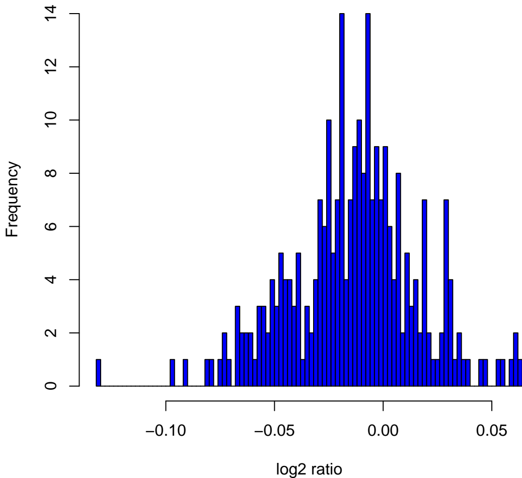
Histogram of log2ratios in 270 HapMap samples at clone Chr15tp-4A11
