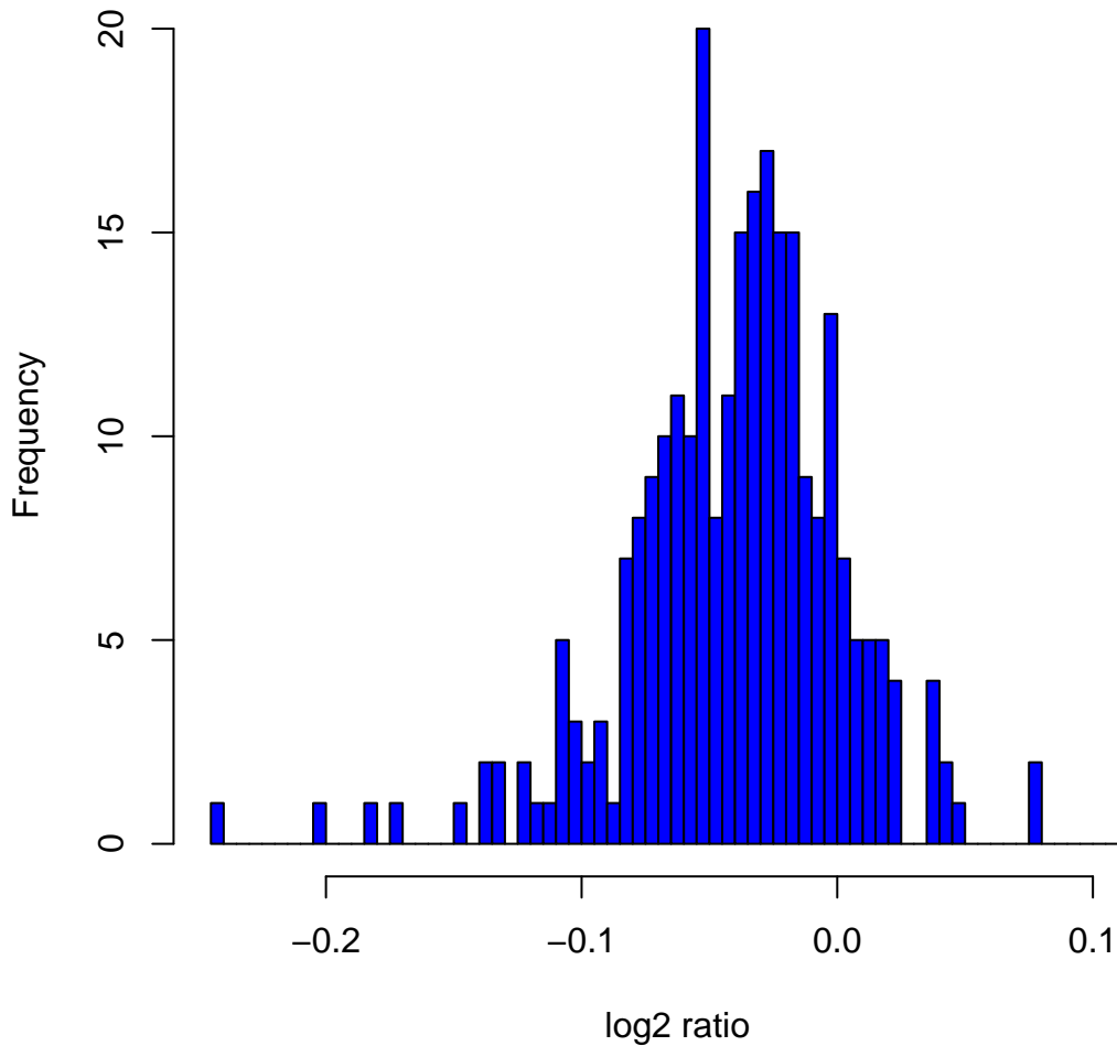
Histogram of log 2 ratios in 270 HapMap samples at clone Chr15tp-4G7
