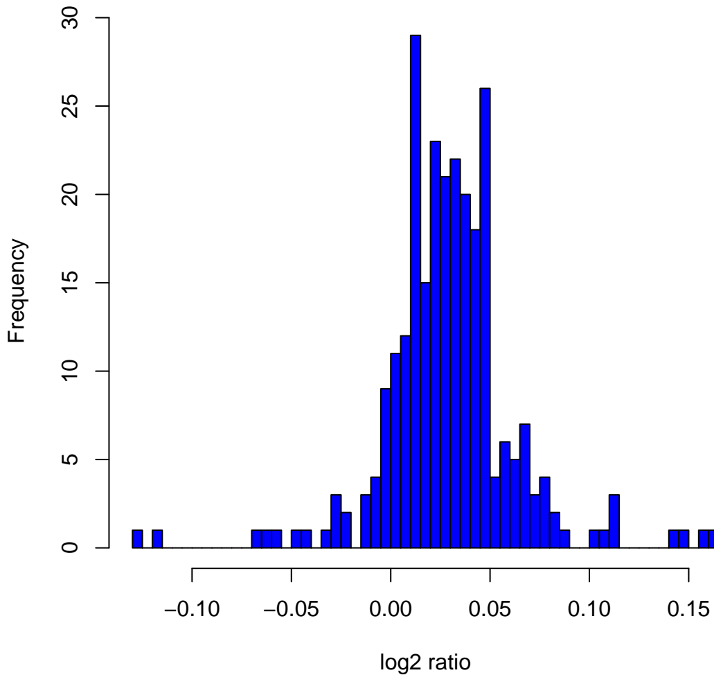
Histogram of log 2 ratios in 270 HapMap samples at clone Chr15tp-5B4
