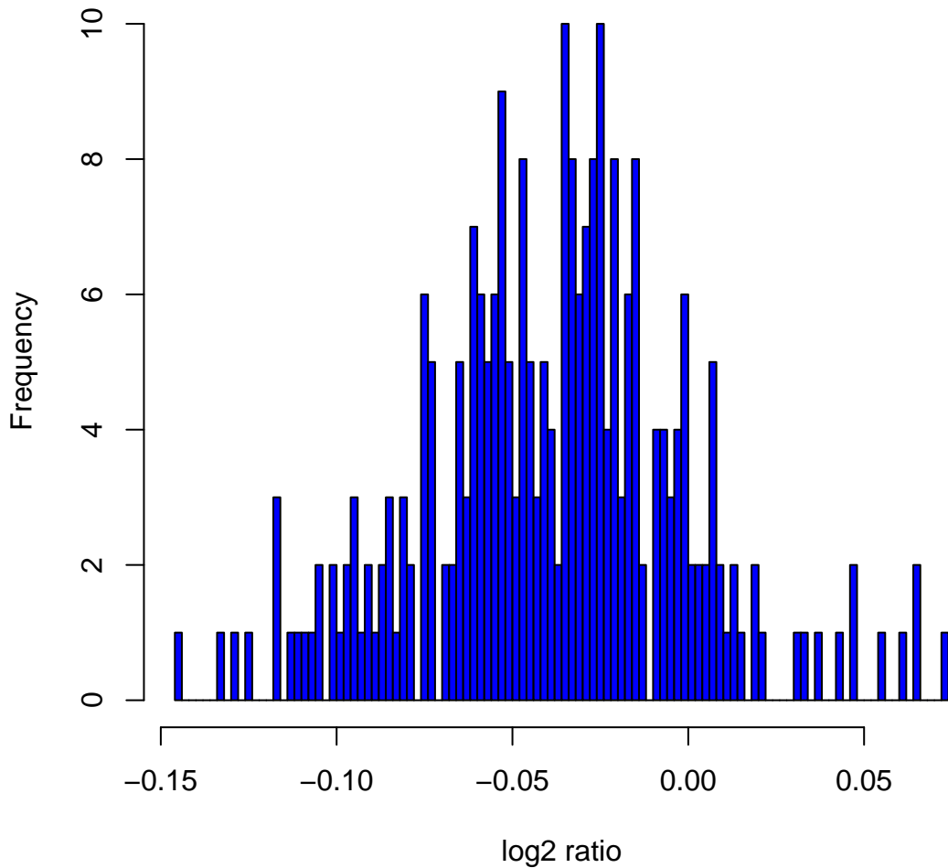
Histogram of log 2 ratios in 270 HapMap samples at clone Chr15tp-5B8
