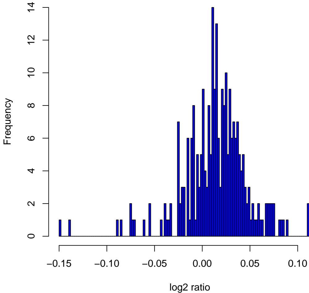
Histogram of log 2 ratios in 270 HapMap samples at clone Chr15tp-5C6
