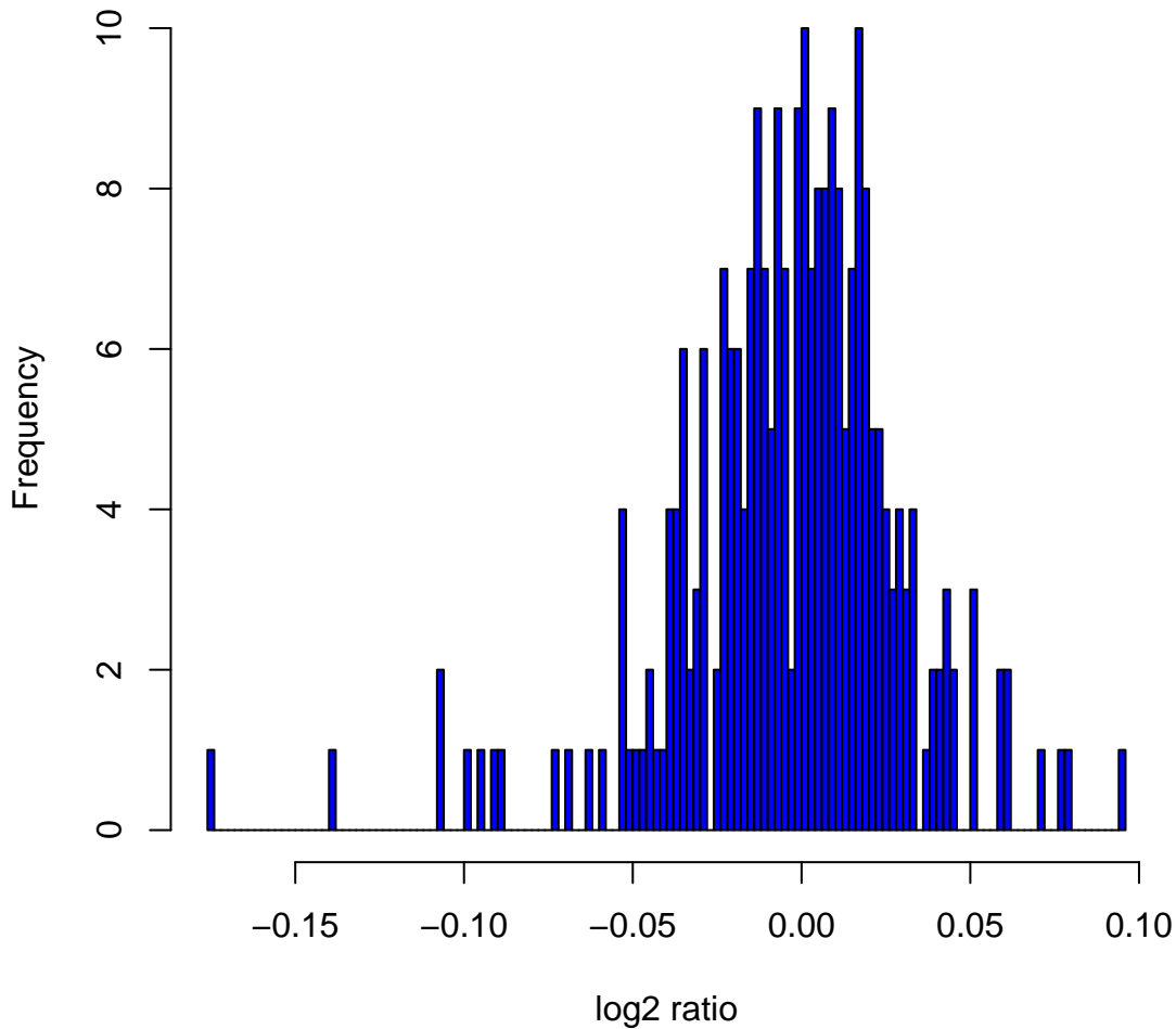
Histogram of log 2 ratios in 270 HapMap samples at clone Chr15tp-5E7
