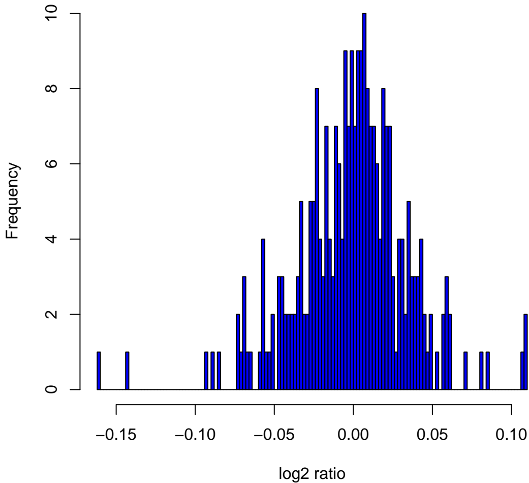
Histogram of log2ratios in 270 HapMap samples at clone Chr15tp-7B10
