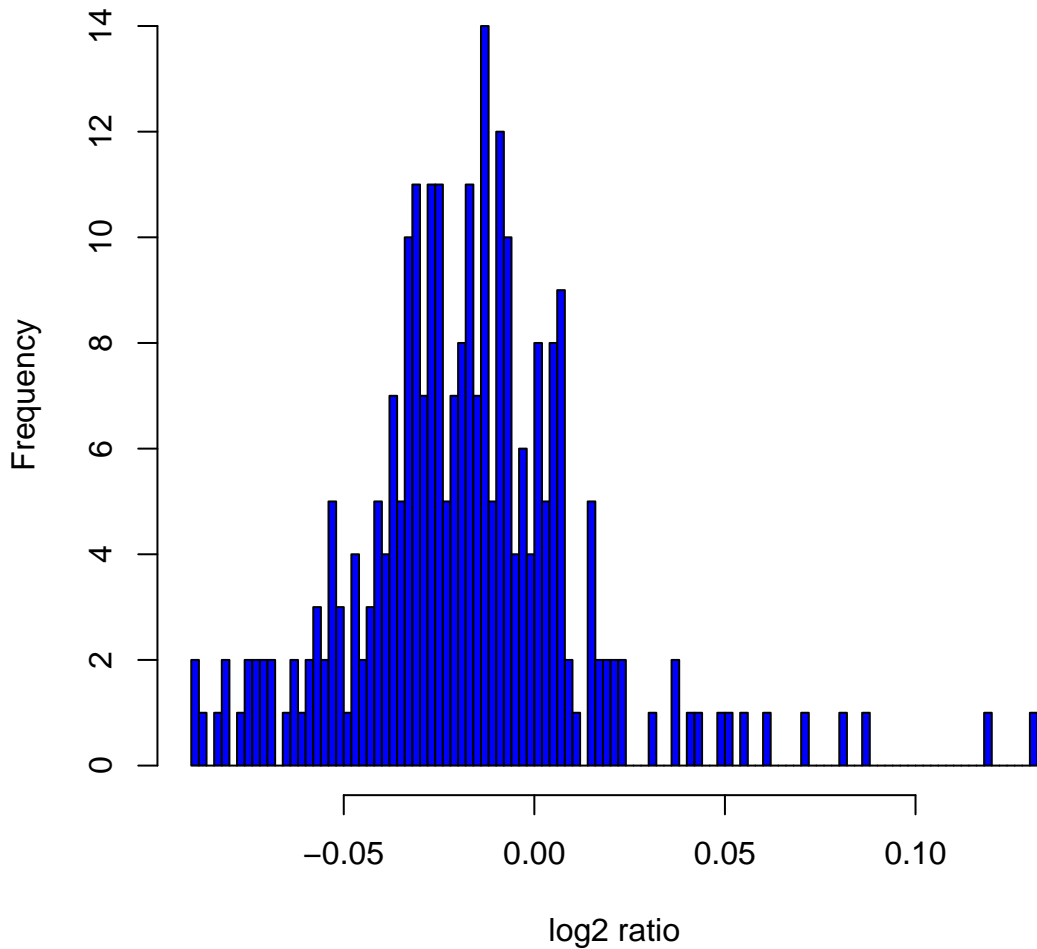
Histogram of log2ratios in 270 HapMap samples at clone Chr15tp-7B12
