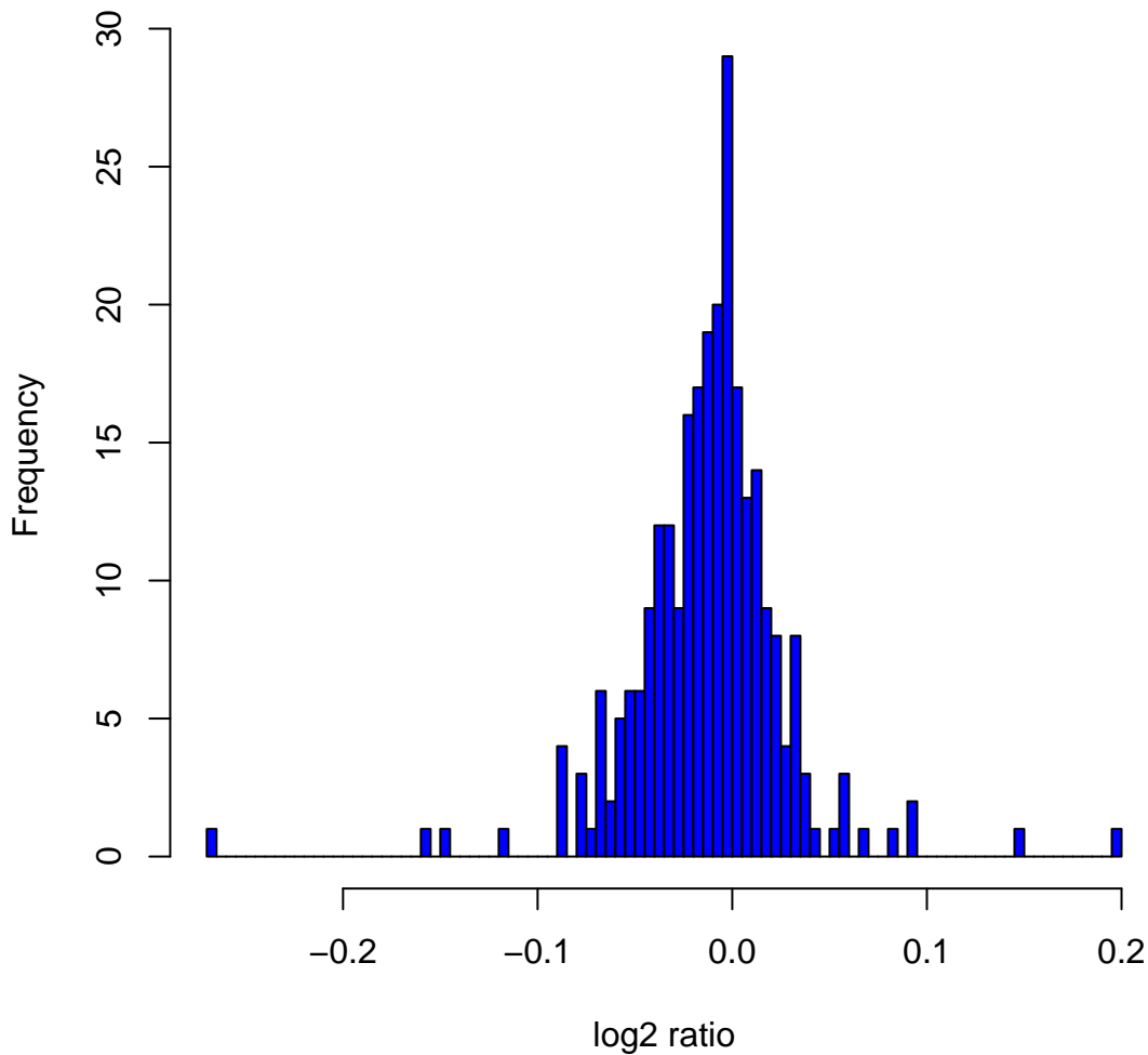
Histogram of log2ratios in 270 HapMap samples at clone Chr15tp-7D10
