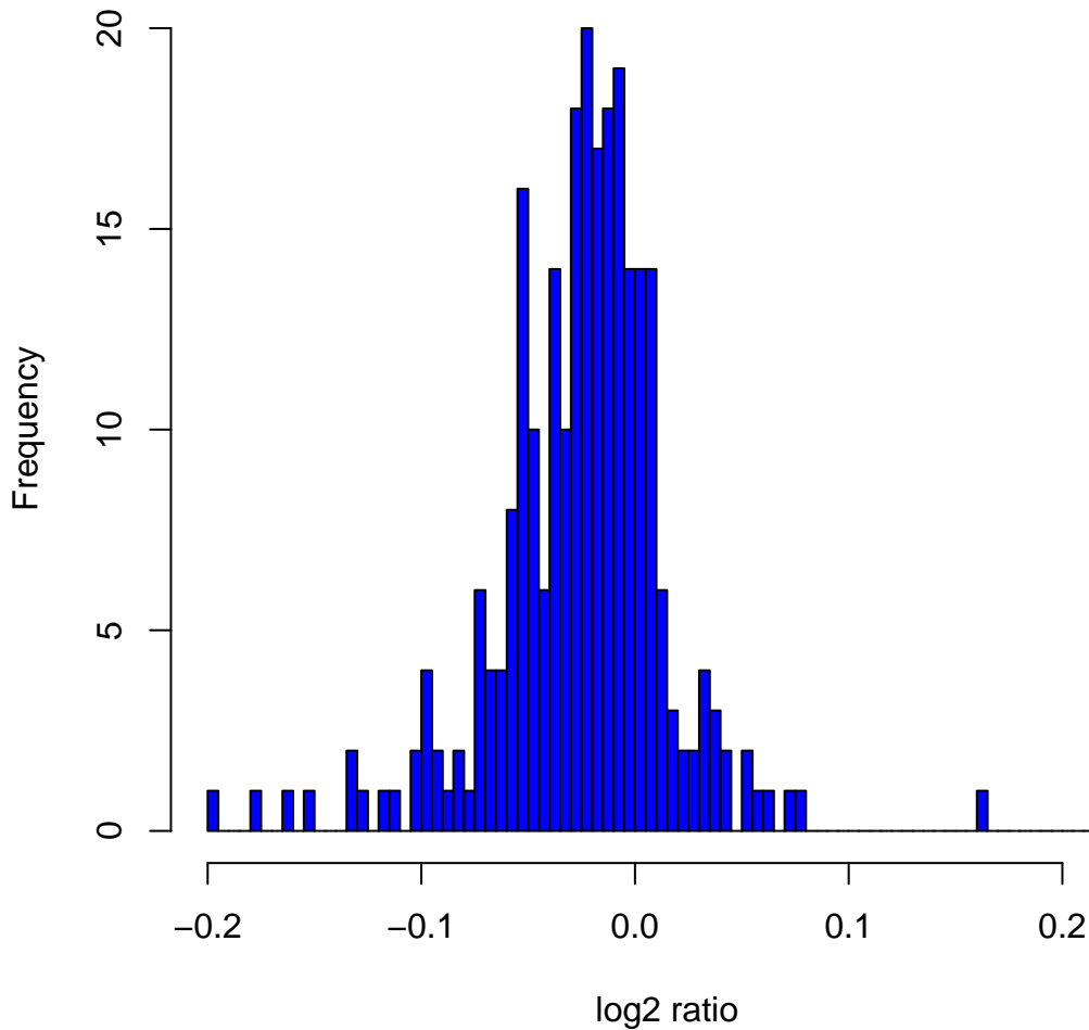
Histogram of \log_2 ratios in 270 HapMap samples at clone Chr15tp-7H9
