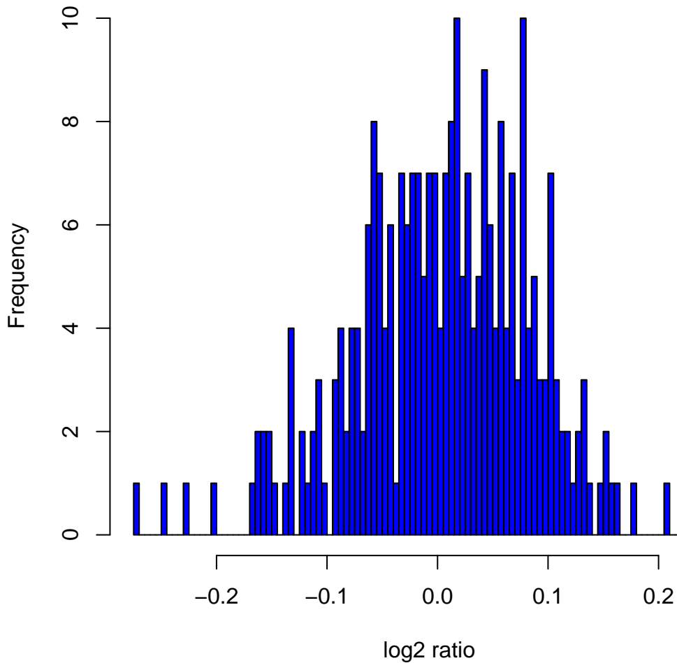
Histogram of \log_2 ratios in 270 HapMap samples at clone Chr15tp-8C10
