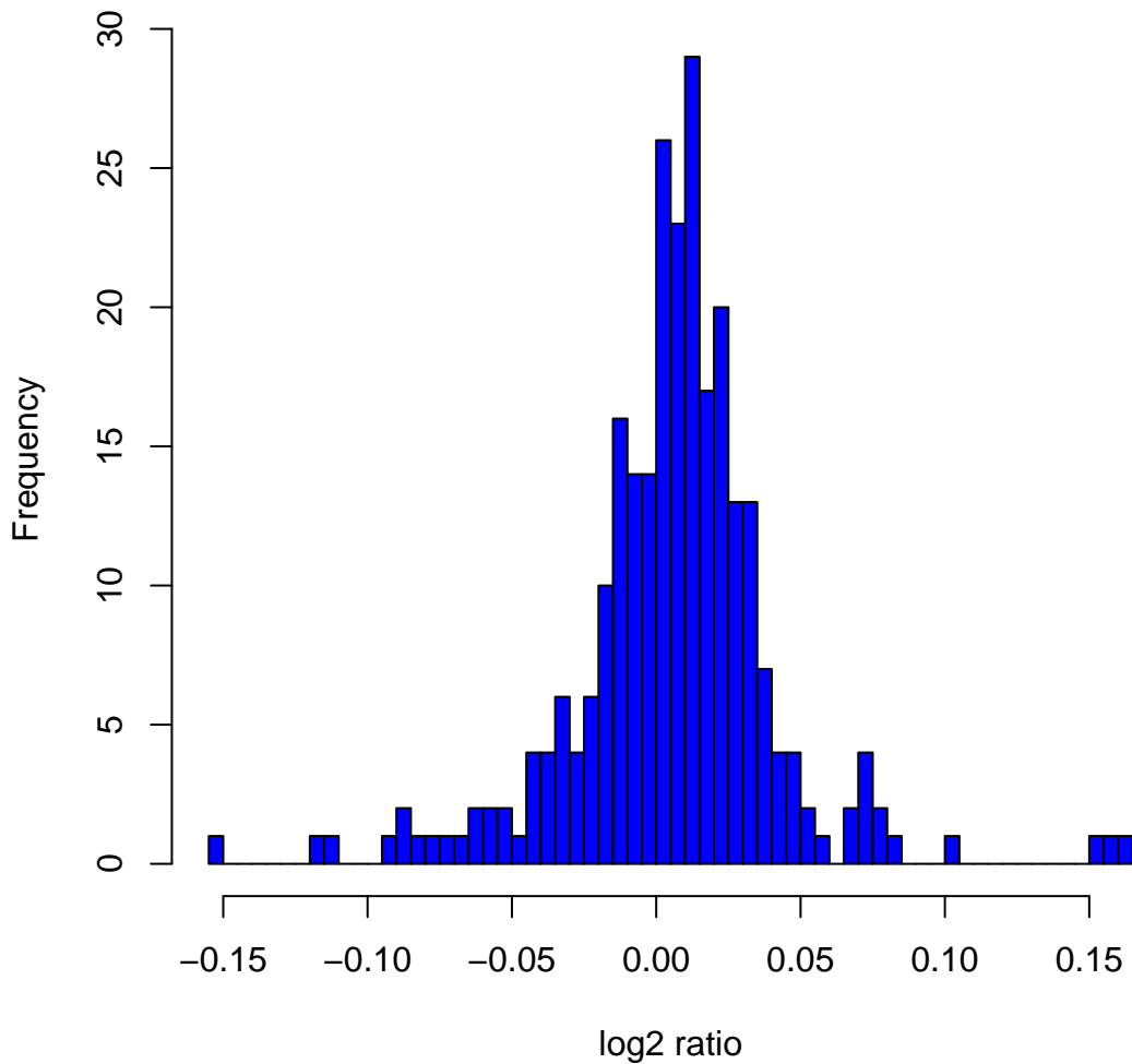
Histogram of log 2 ratios in 270 HapMap samples at clone Chr15tp-9C3
