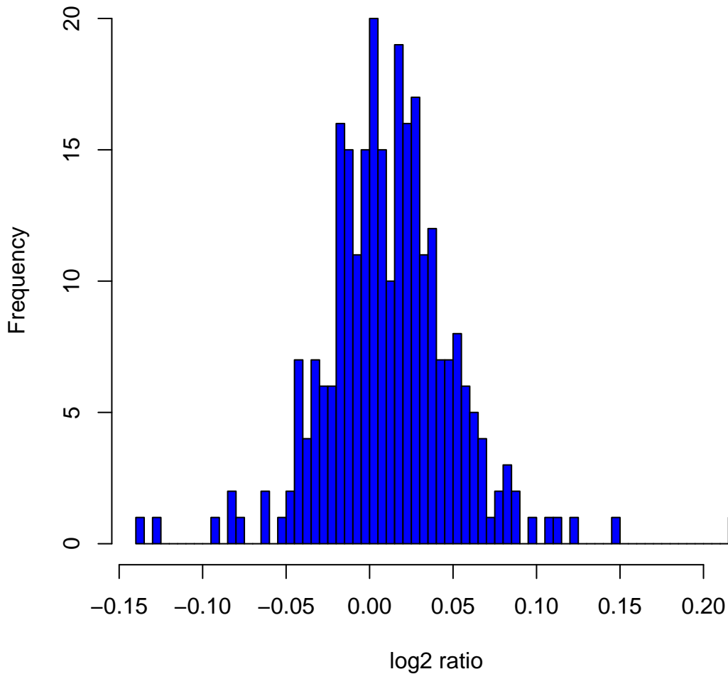
Histogram of log2ratios in 270 HapMap samples at clone Chr15tp-9E12
