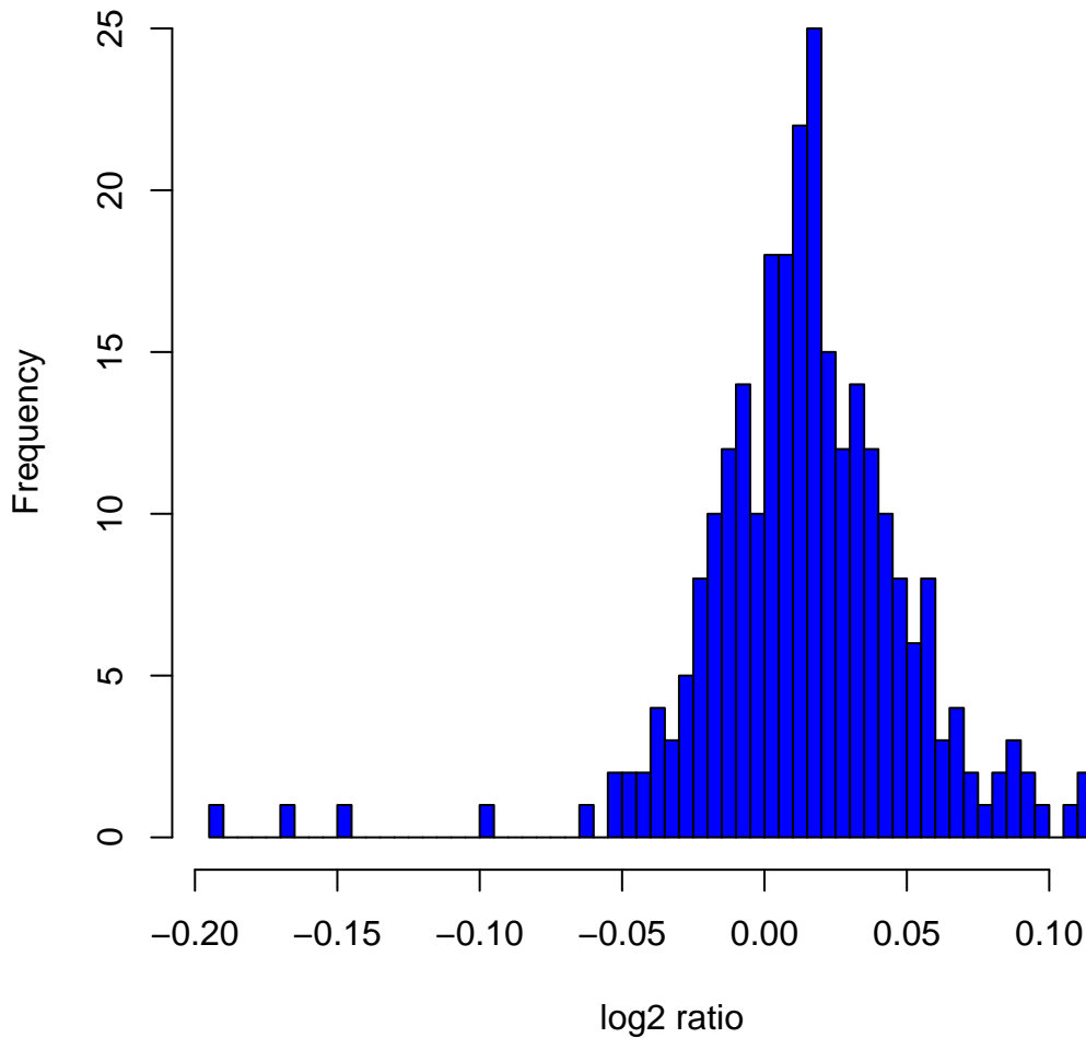
Histogram of log2ratios in 270 HapMap samples at clone Chr16tp-11A10
