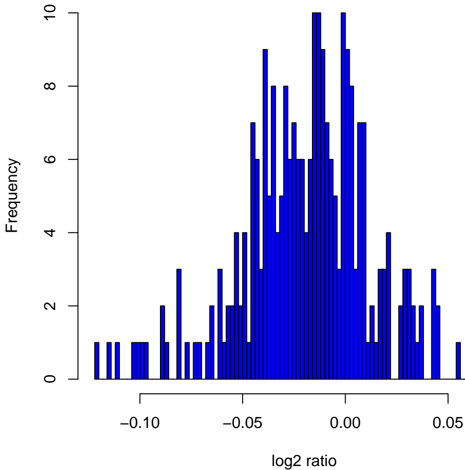
Histogram of log2ratios in 270 HapMap samples at clone Chr16tp-11B5
