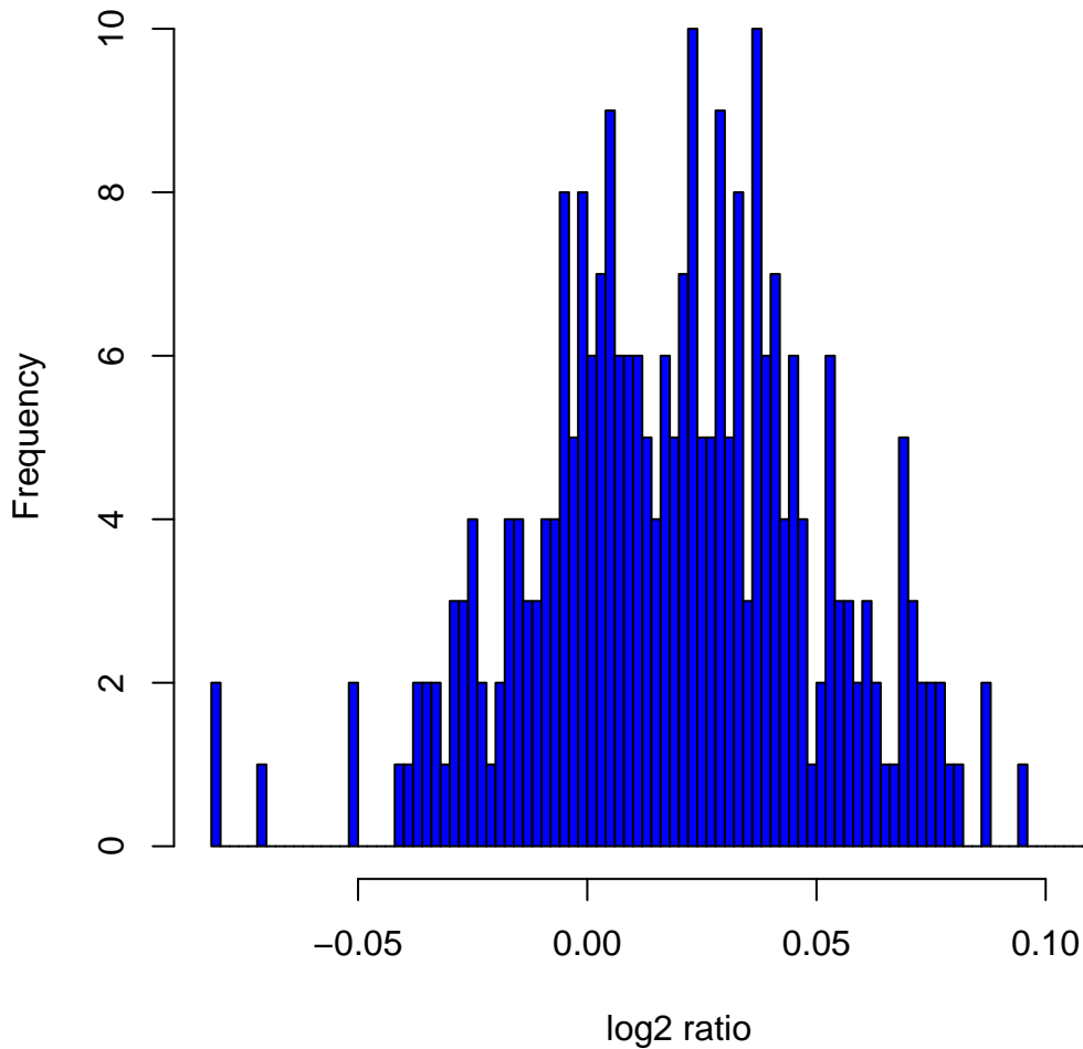
Histogram of log2ratios in 270 HapMap samples at clone Chr16tp-11D3
