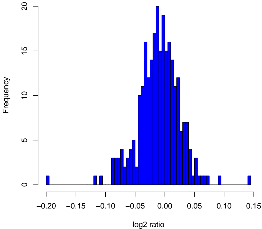
Histogram of log2ratios in 270 HapMap samples at clone Chr16tp-11H8
