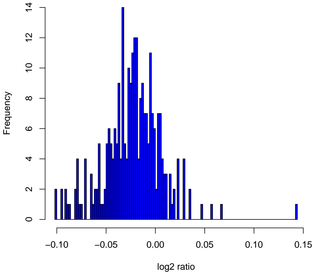
Histogram of log2ratios in 270 HapMap samples at clone Chr16tp-12A7
