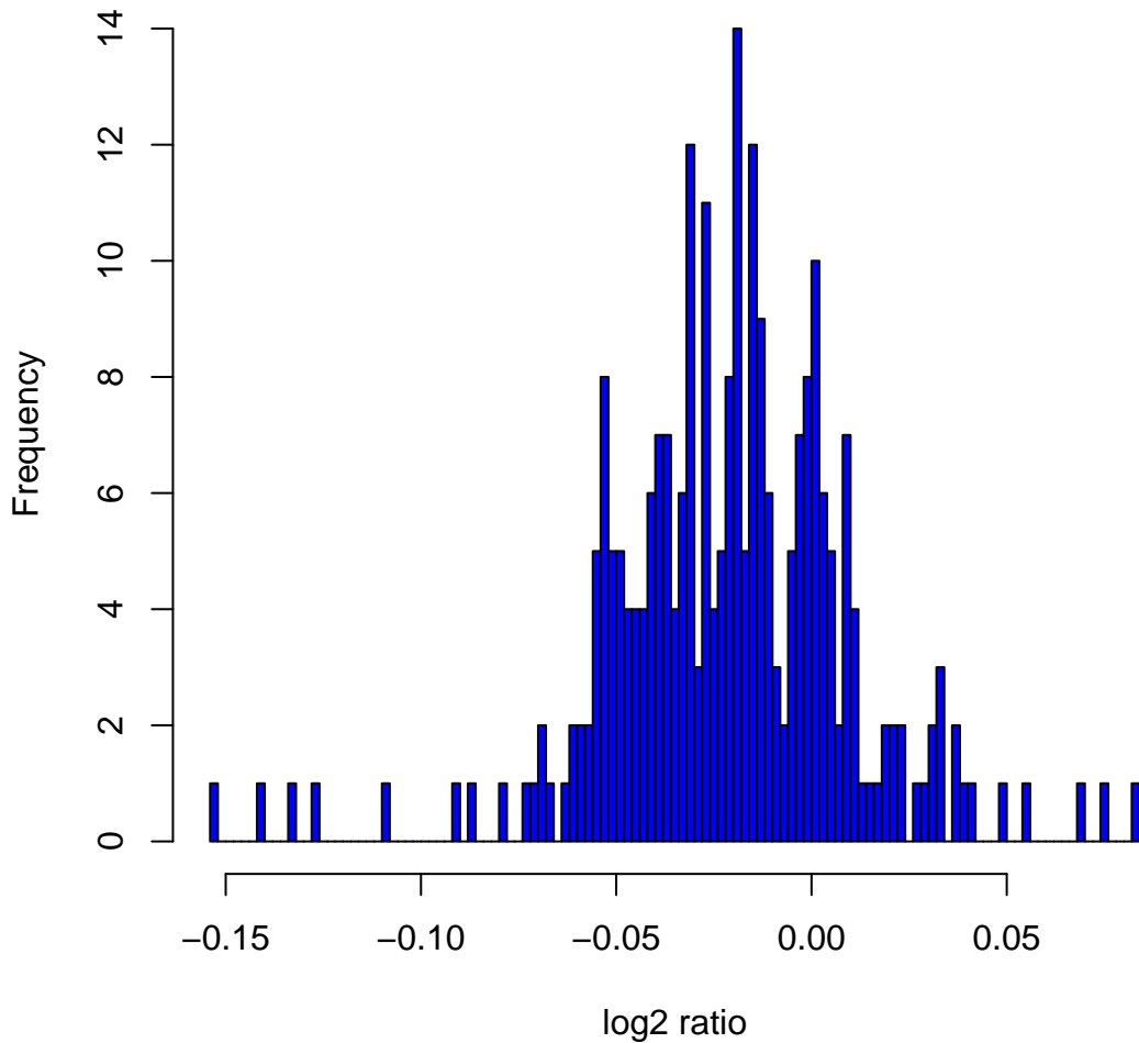
Histogram of log2ratios in 270 HapMap samples at clone Chr16tp-12B1
