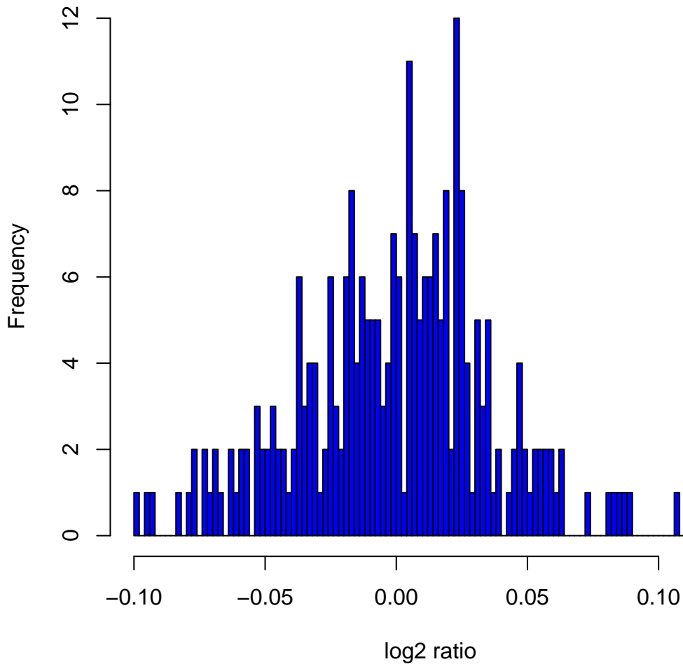
Histogram of log2ratios in 270 HapMap samples at clone Chr16tp-12B6
