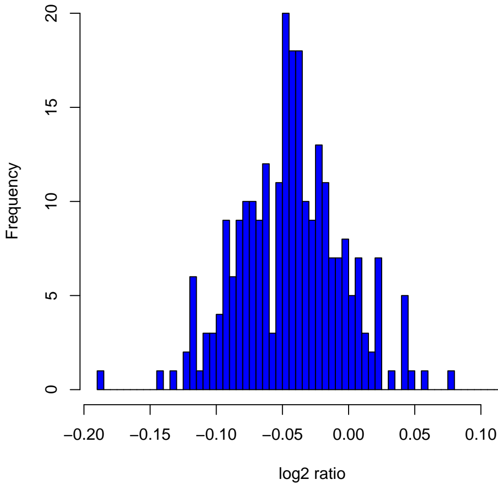
Histogram of log2ratios in 270 HapMap samples at clone Chr16tp-12B7
