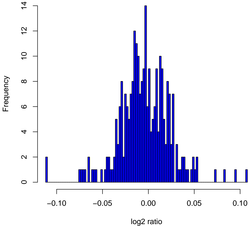
Histogram of log2ratios in 270 HapMap samples at clone Chr16tp-12C1
