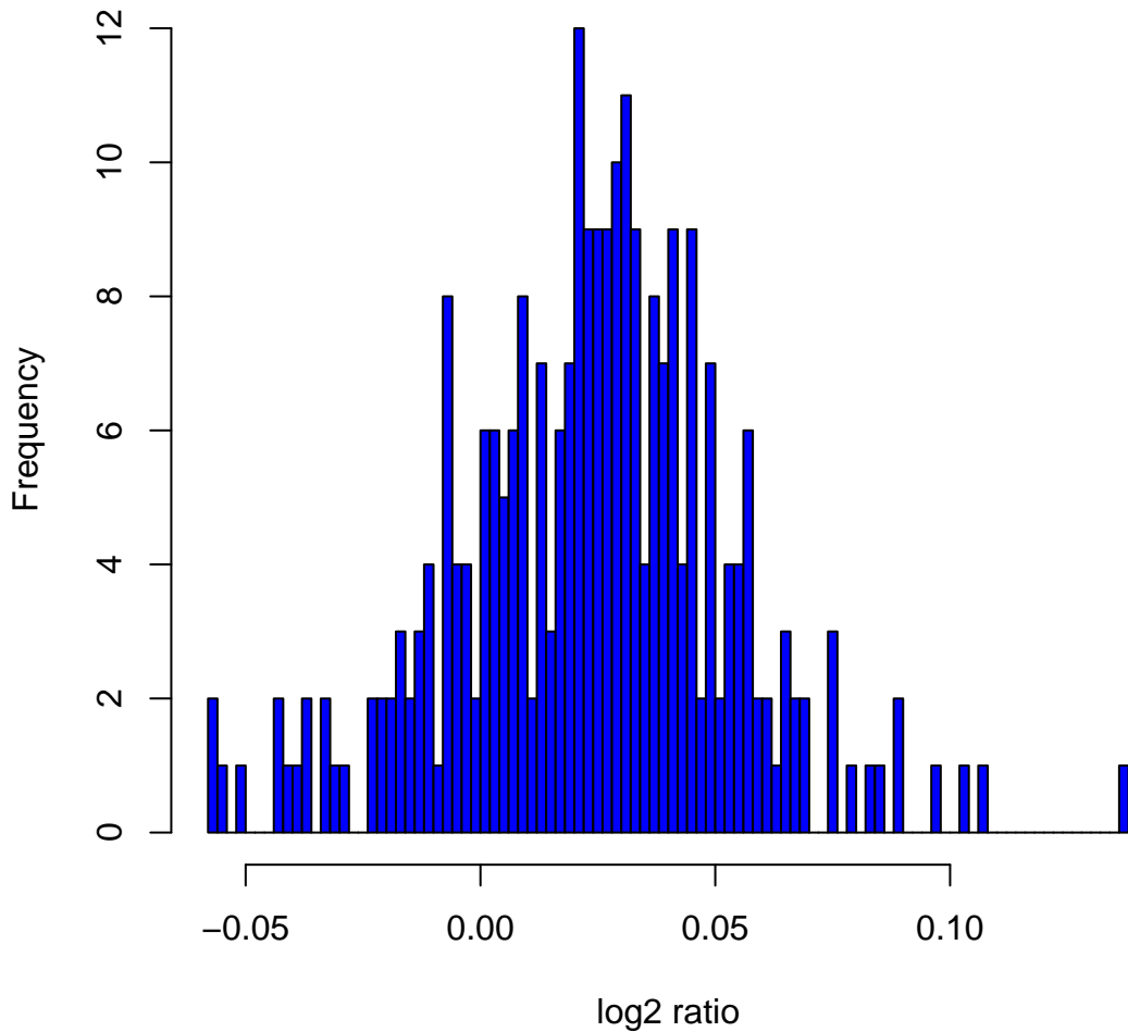
Histogram of log2ratios in 270 HapMap samples at clone Chr16tp-12C7
