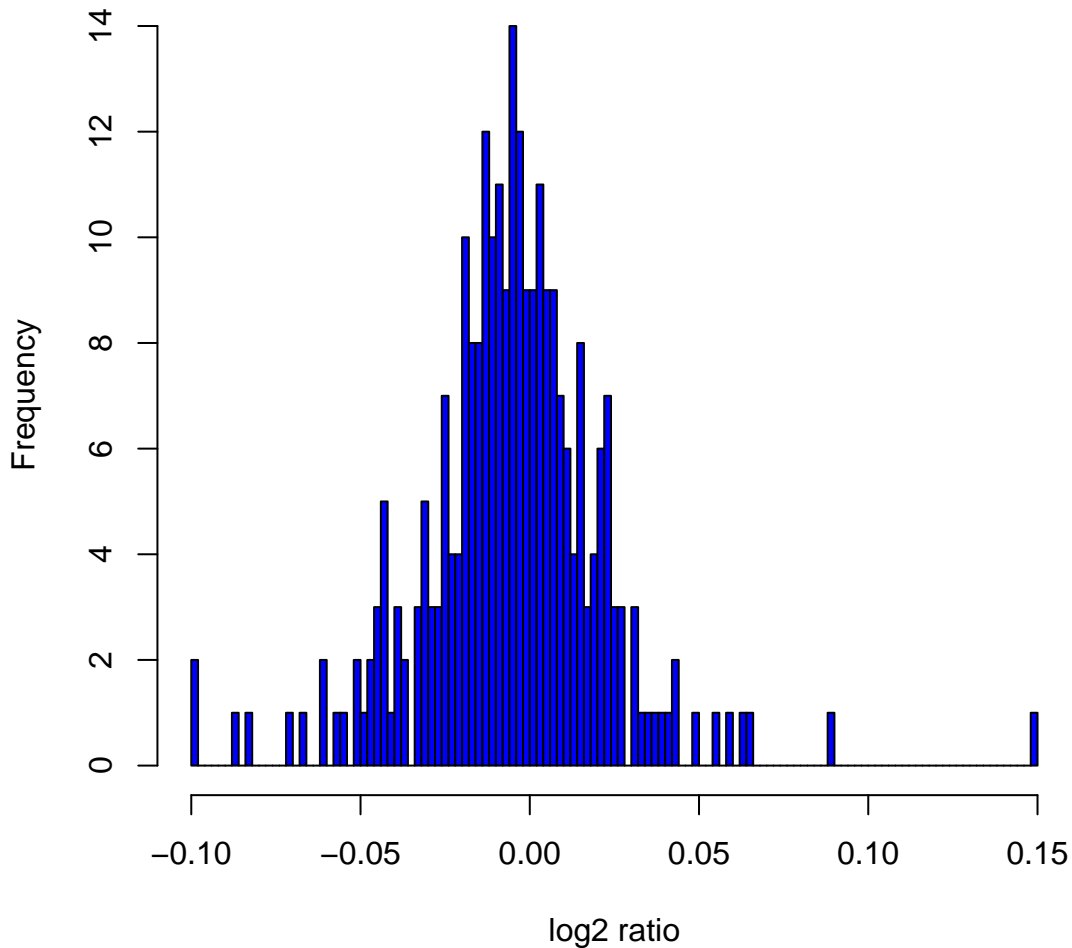
Histogram of log2ratios in 270 HapMap samples at clone Chr16tp-12G10
