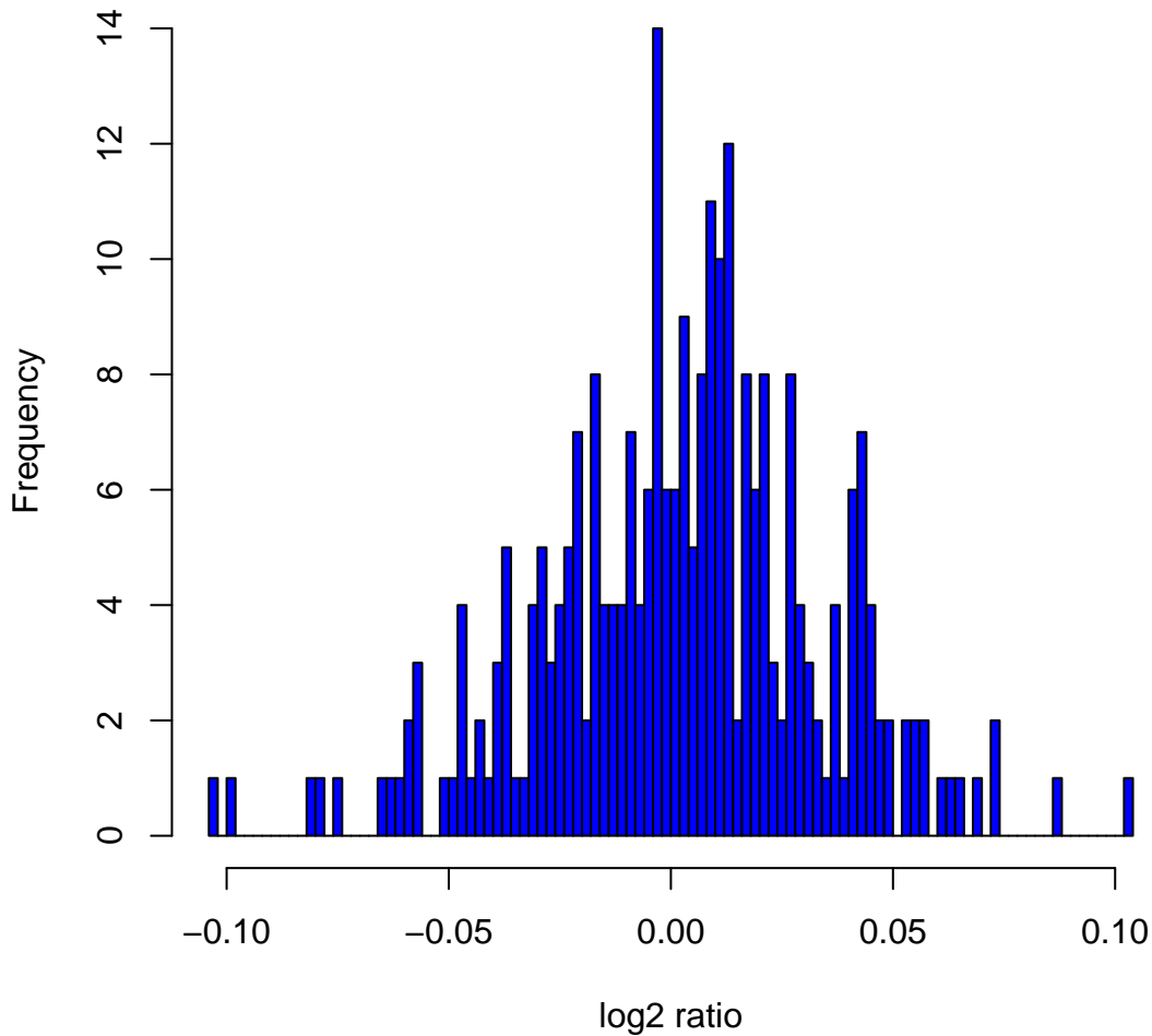
Histogram of log2ratios in 270 HapMap samples at clone Chr16tp-13C2
