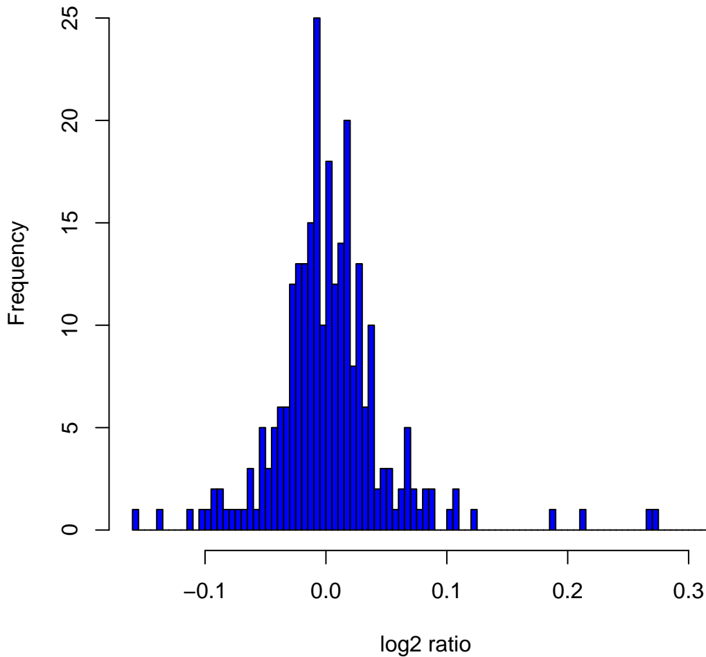
Histogram of log2ratios in 270 HapMap samples at clone Chr16tp-13D2
