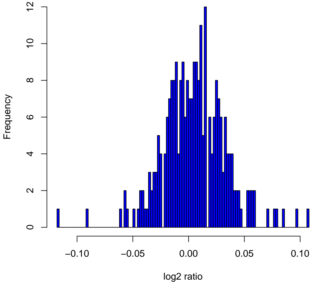
Histogram of log 2 ratios in 270 HapMap samples at clone Chr16tp-1B7
