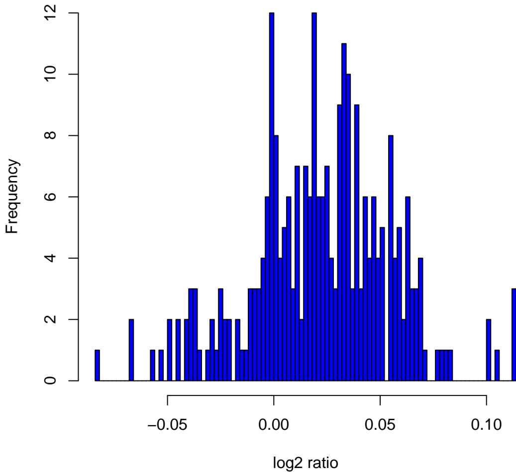
Histogram of log2ratios in 270 HapMap samples at clone Chr16tp-1D12
