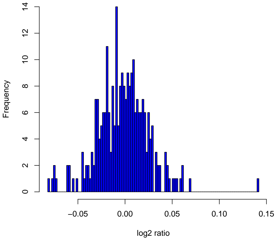
Histogram of log2ratios in 270 HapMap samples at clone Chr16tp-1E5
