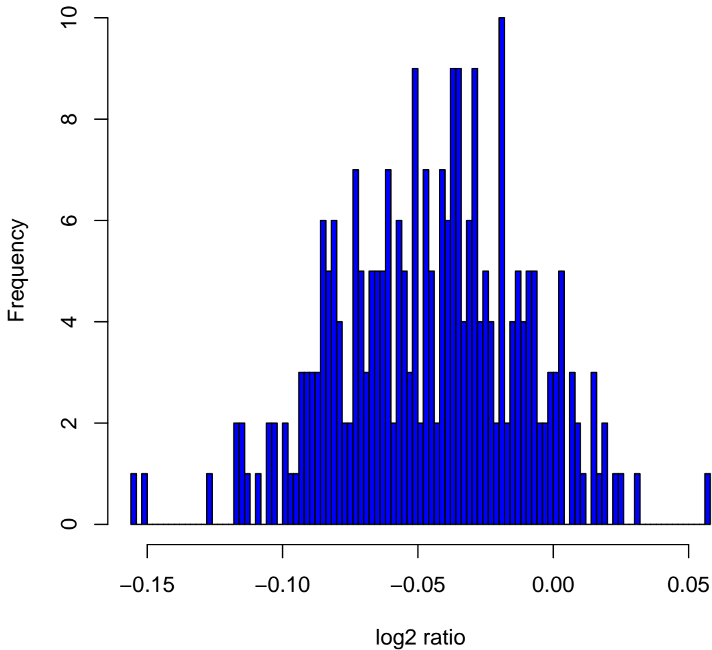
Histogram of log2ratios in 270 HapMap samples at clone Chr16tp-1H10
