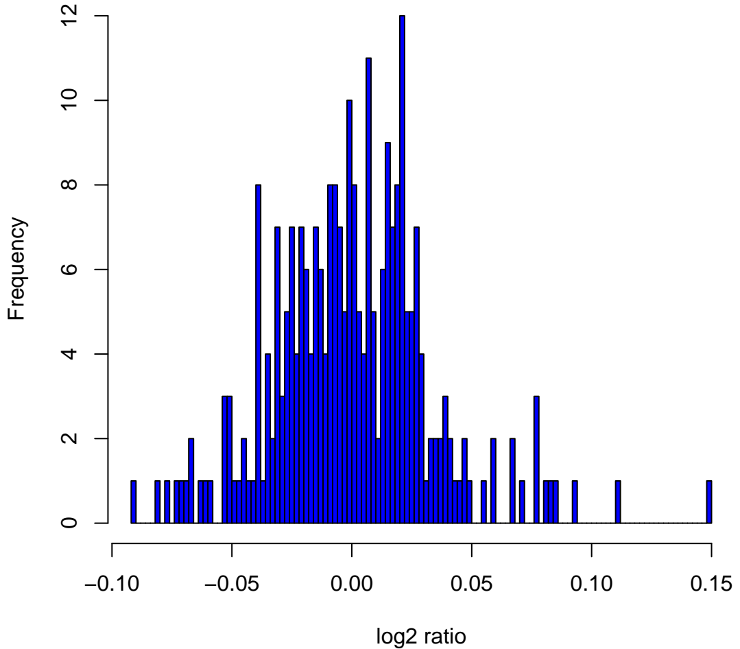
Histogram of log2ratios in 270 HapMap samples at clone Chr16tp-2A11
