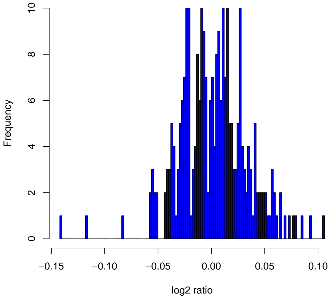
Histogram of log 2 ratios in 270 HapMap samples at clone Chr16tp-2A7
