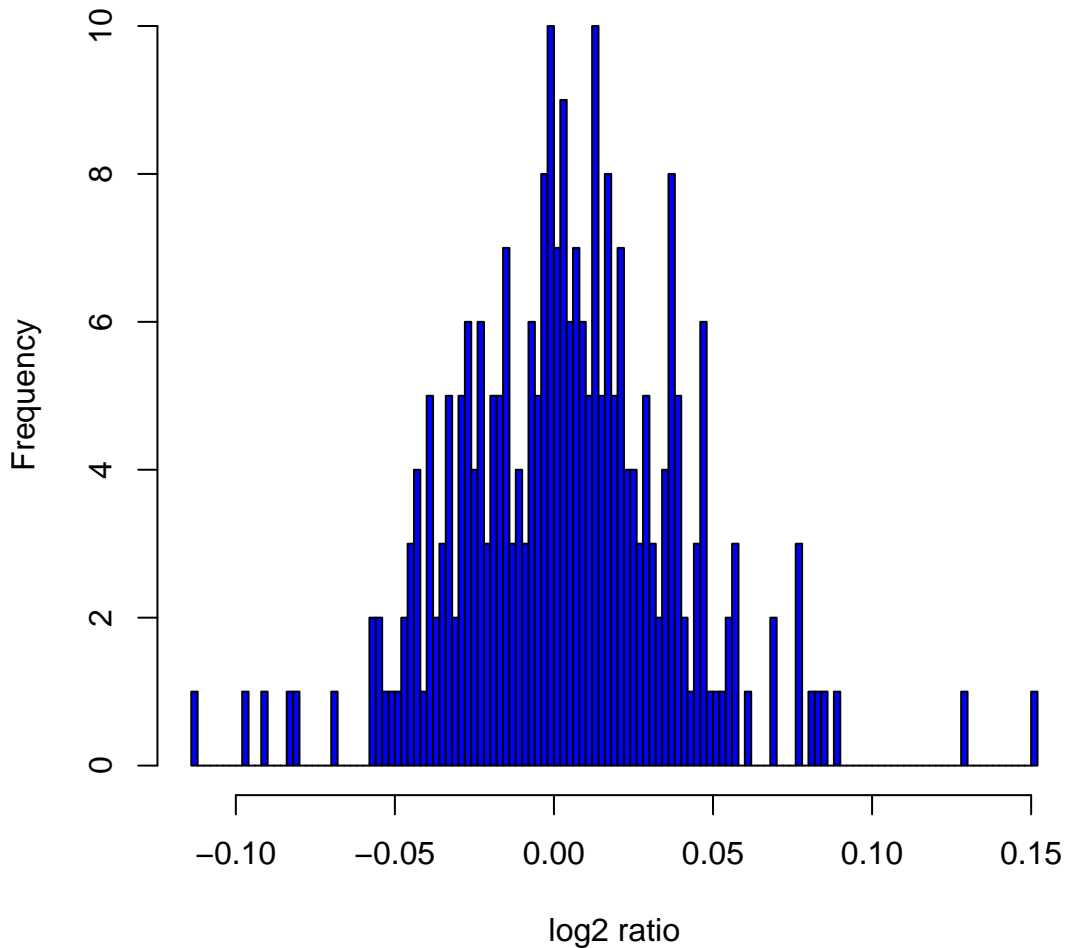
Histogram of log2ratios in 270 HapMap samples at clone Chr16tp-3A7
