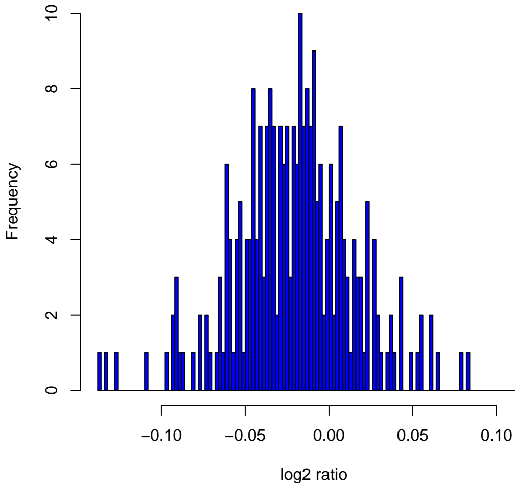
Histogram of \log_2 ratios in 270 HapMap samples at clone Chr16tp-3B3
