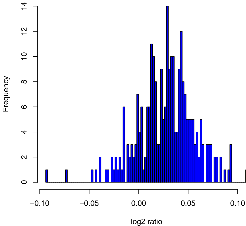
Histogram of log2ratios in 270 HapMap samples at clone Chr16tp-3C12
