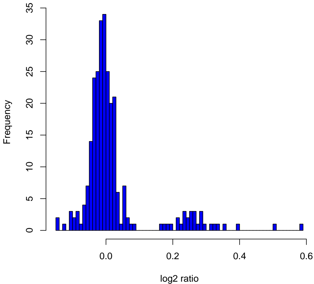
Histogram of log 2 ratios in 270 HapMap samples at clone Chr16tp-3C5
