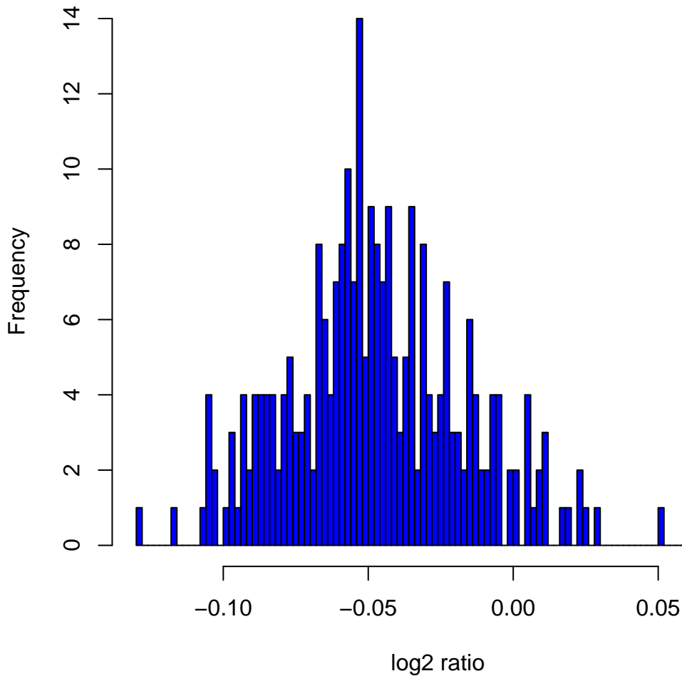
Histogram of log 2 ratios in 270 HapMap samples at clone Chr16tp-3C7
