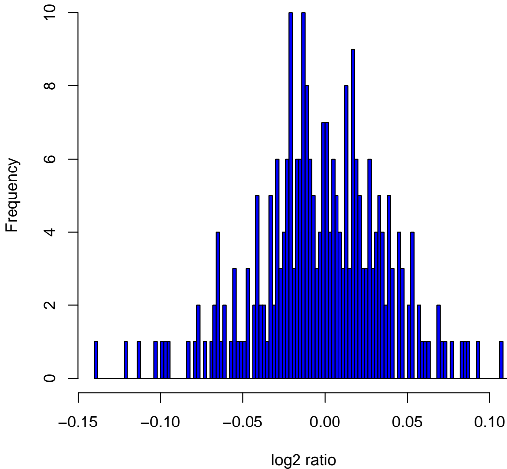
Histogram of log2ratios in 270 HapMap samples at clone Chr16tp-3D7
