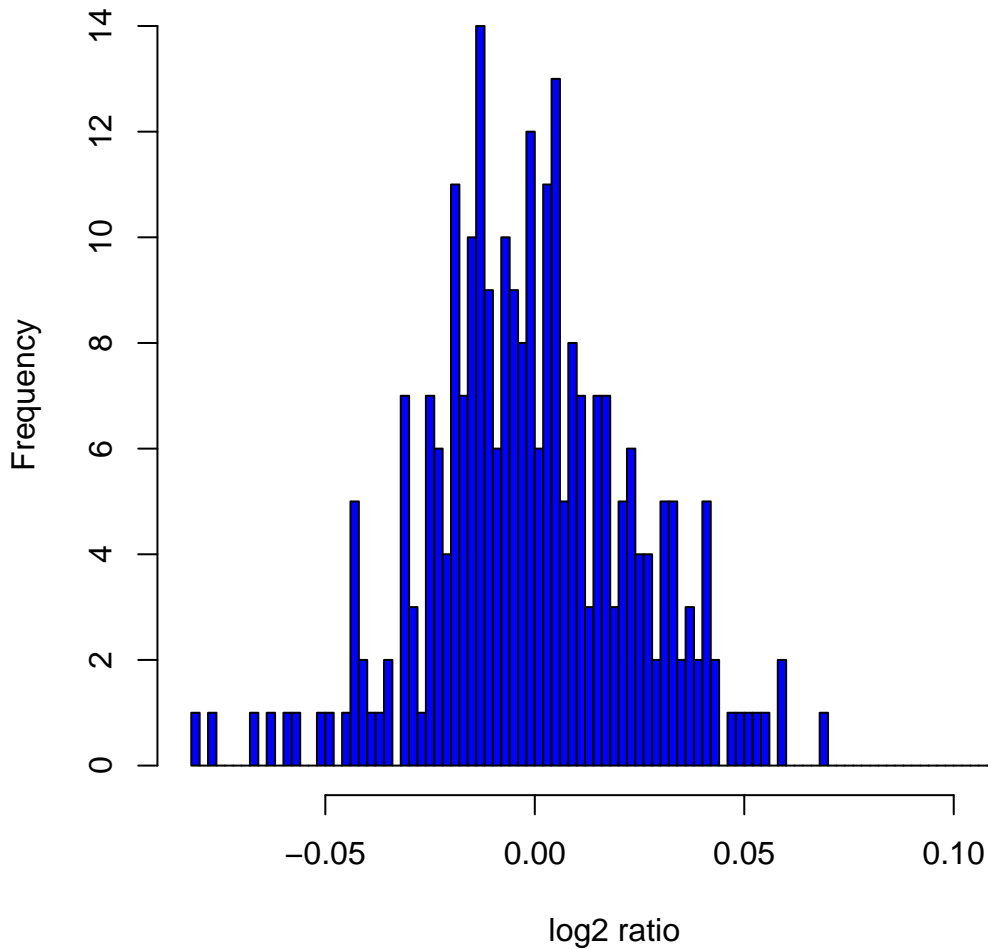
Histogram of log 2 ratios in 270 HapMap samples at clone Chr16tp-3E8
