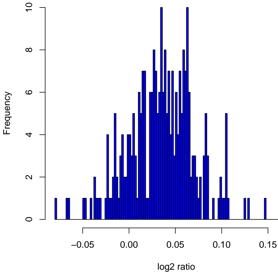
Histogram of \log_2 ratios in 270 HapMap samples at clone Chr16tp-3G6
