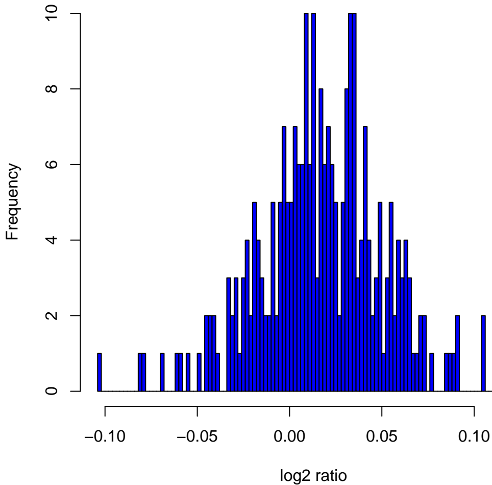
Histogram of \log_2 ratios in 270 HapMap samples at clone Chr16tp-3G7
