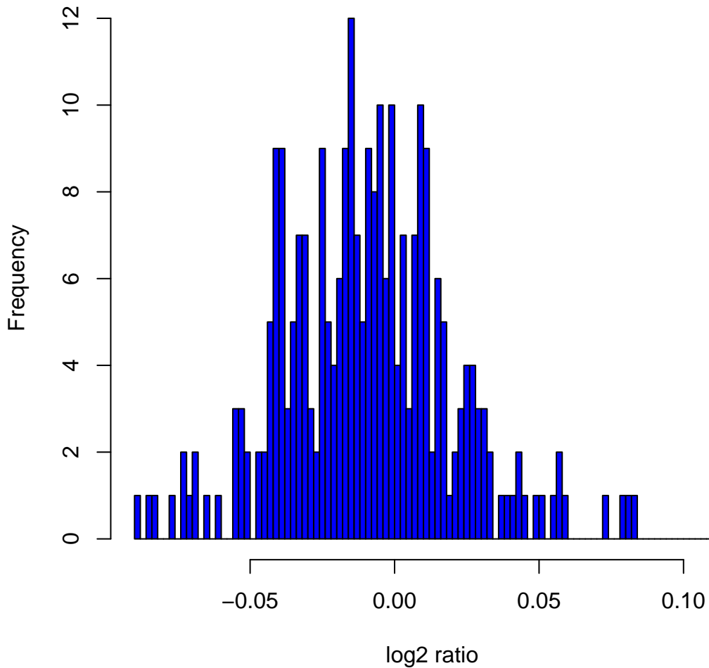
Histogram of log2ratios in 270 HapMap samples at clone Chr16tp-4A11
