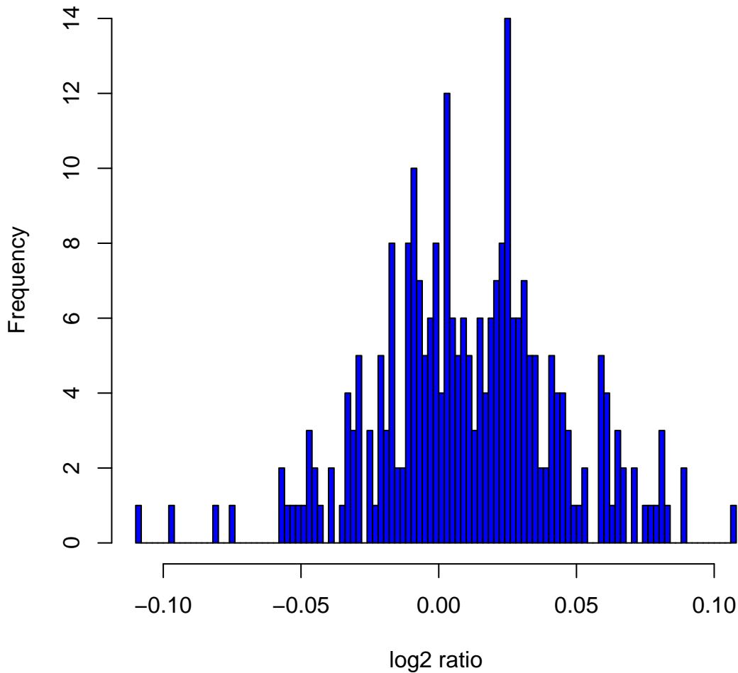
Histogram of log 2 ratios in 270 HapMap samples at clone Chr16tp-4B8
