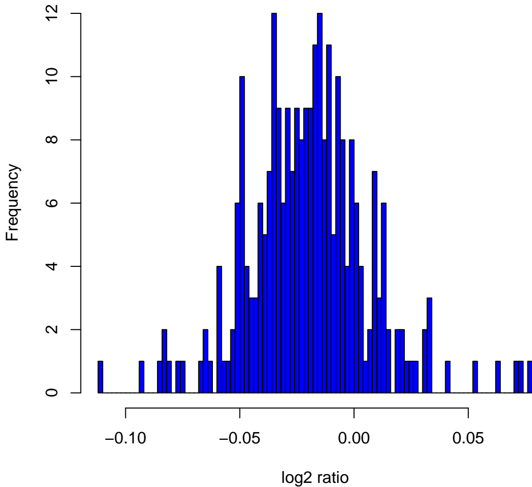
Histogram of log 2 ratios in 270 HapMap samples at clone Chr16tp-4C7
