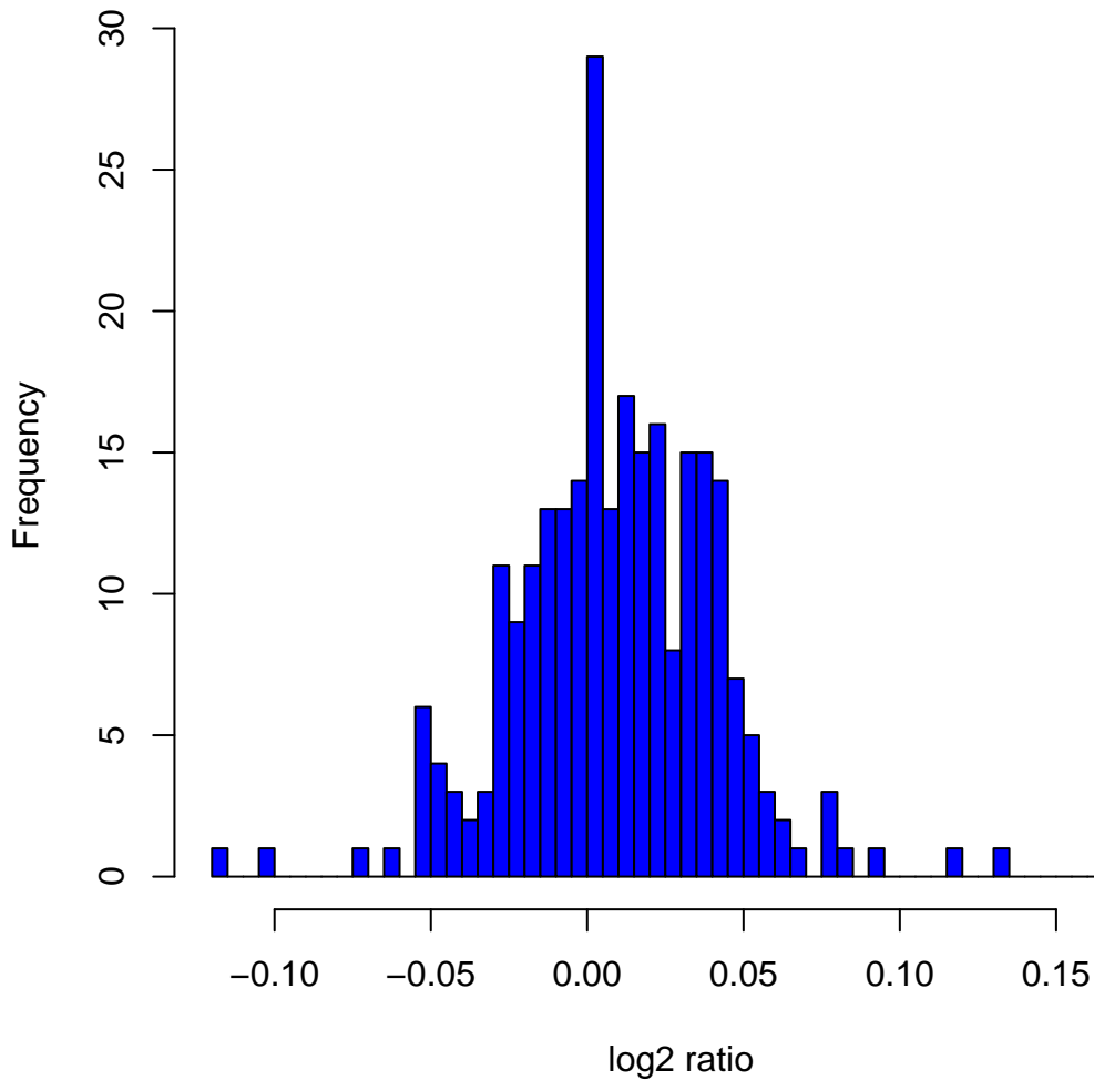
Histogram of \log_2 ratios in 270 HapMap samples at clone Chr16tp-4D7
