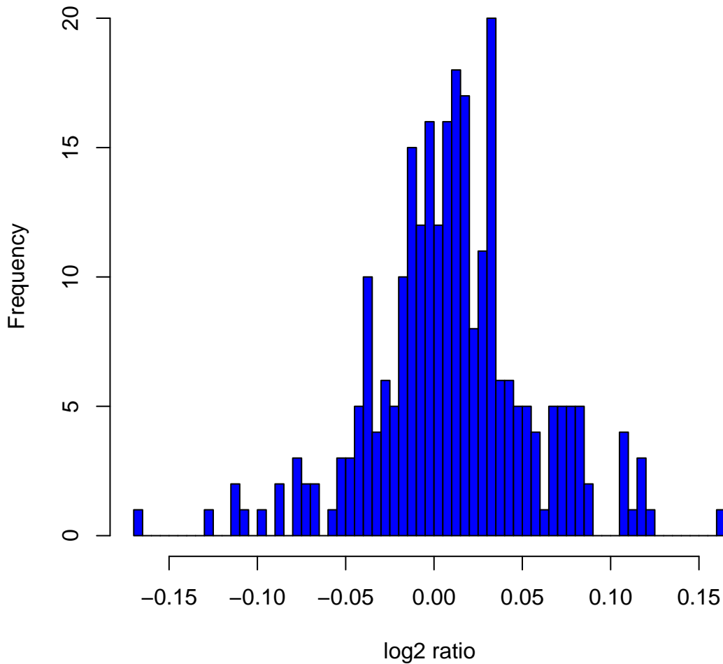
Histogram of log2ratios in 270 HapMap samples at clone Chr16tp-8A10
