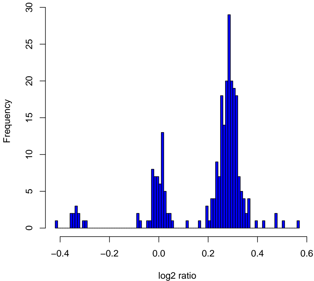
Histogram of log2ratios in 270 HapMap samples at clone Chr16tp-8B1
