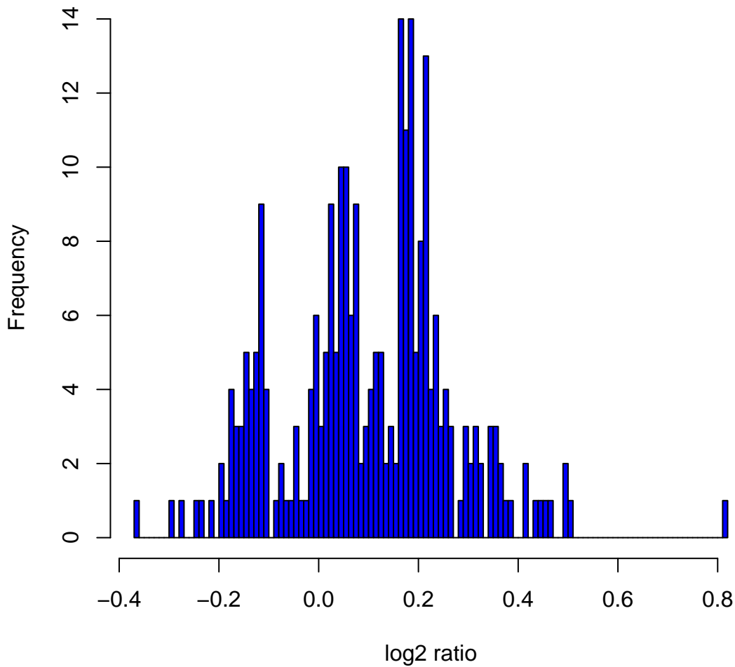
Histogram of log 2 ratios in 270 HapMap samples at clone Chr16tp-8C5
